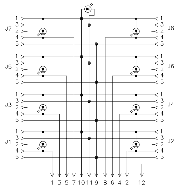
P1 WIRING DIAGRAM
